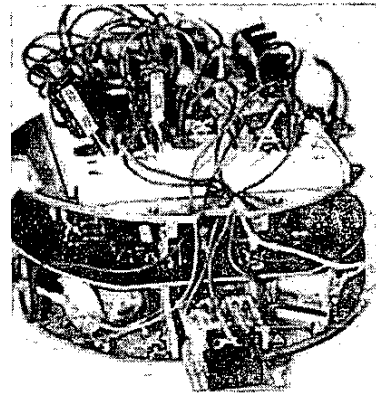
Fig. 2: Graymark robot with bread boarded "whiskers."
